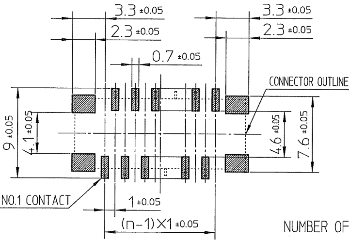
RECOMMENDED PC BOARD LAYOUT (COMPONENT SIDE)
