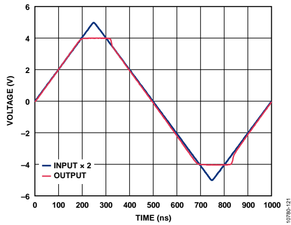
Figure 21. Overdrive Recovery, G = 2
