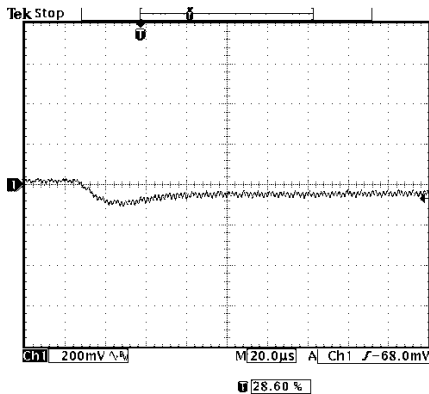
Vout=3.3V 50% to 100% load transients at 12.0V input and Ta=25° C
