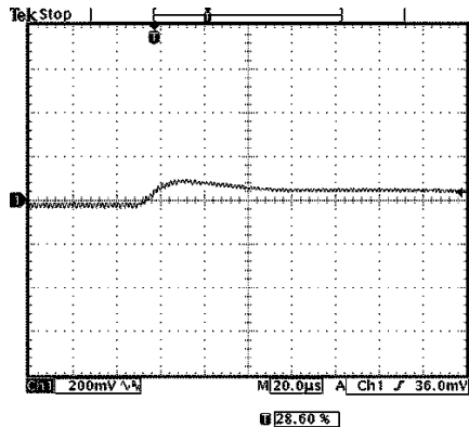
Vout=3.3V 100% to 50% load transients at 12.0V input and Ta=25° C
