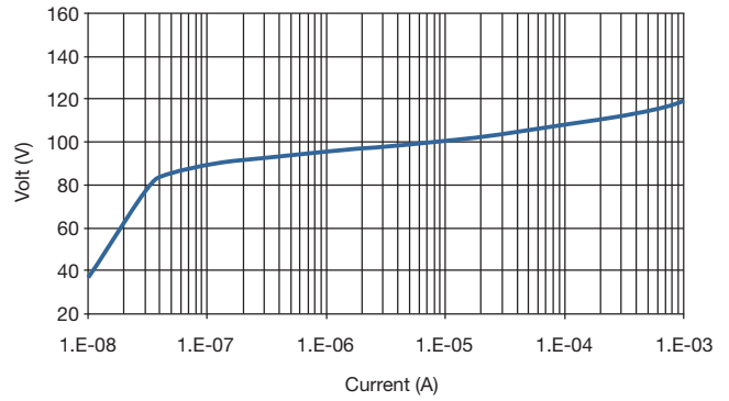
V/I Curve - SPV
