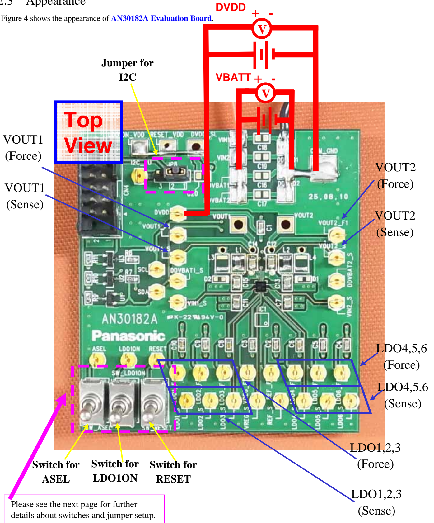
Figure 4. Appearance of AN30182A Evaluation Board (Top View)
