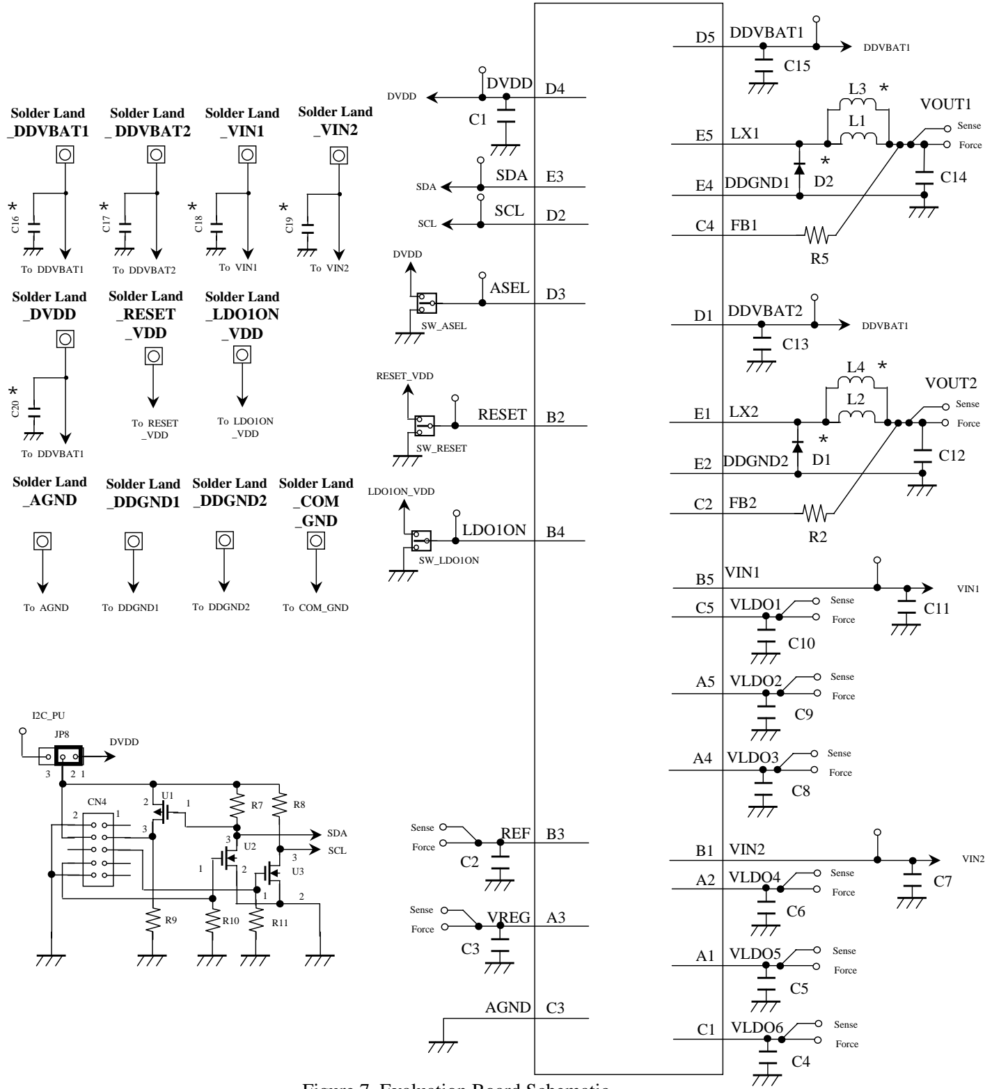
Figure 7. Evaluation Board Schematic
