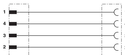
Contact assignment of M12 plugs / M8 sockets
