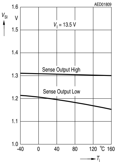
Sense Threshold V_{SI} versus Temperature T_j
