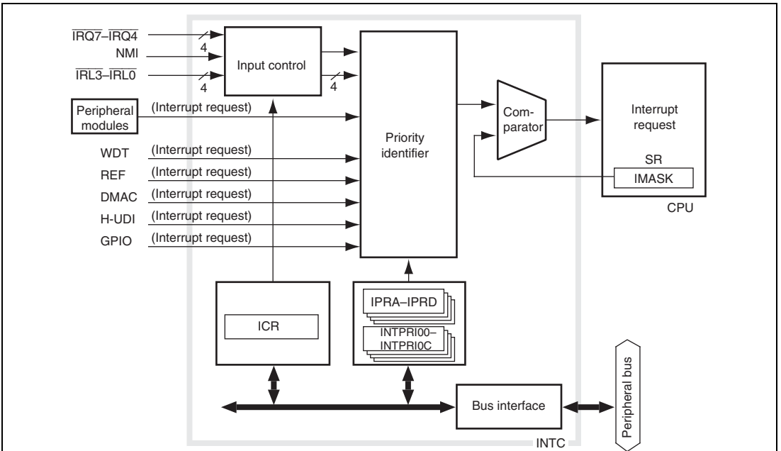
Figure 9.1 shows a block diagram of the INTC.
