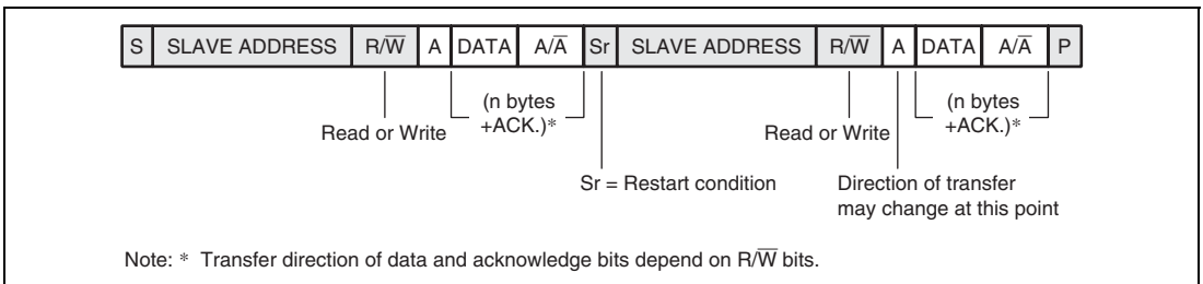
Figure 19.5 Combination Transfer Format of Master Transfer
