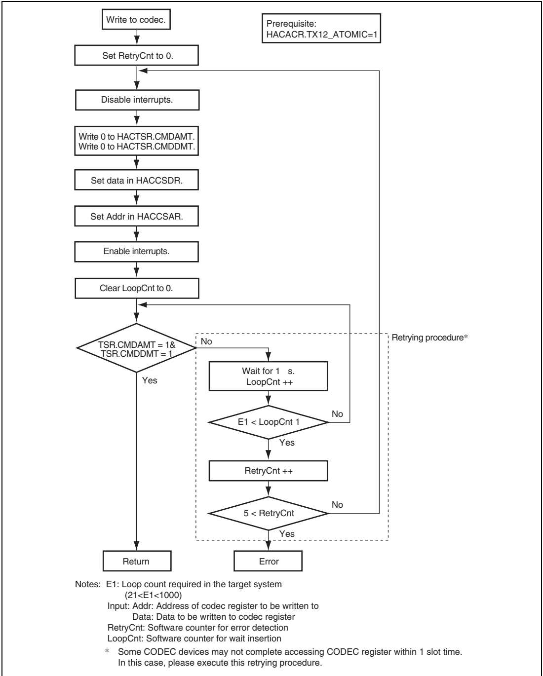
Figure 25.4 Sample Flowchart for Off-Chip Codec Register Write
