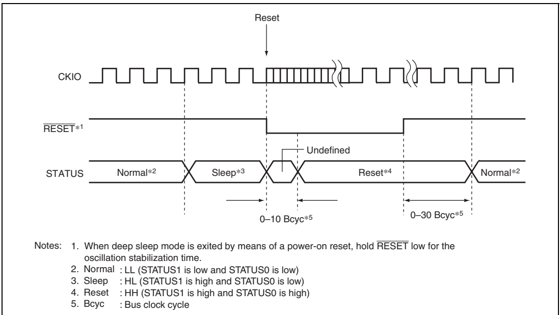
Figure 14.10 STATUS Output in Sequence of Deep Sleep → Power-On Reset
