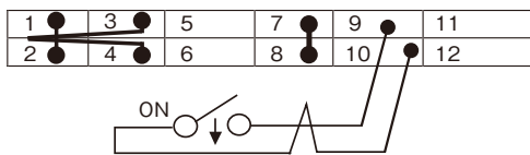
Connecting circuit with CN01 or CN02 connector
