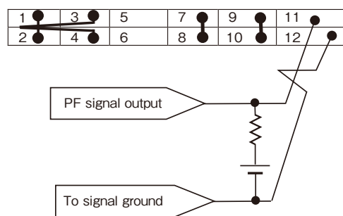
Connecting circuit with CN01 or CN02 connector
