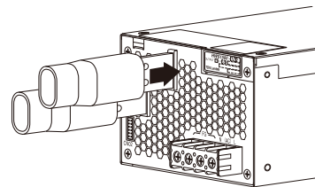
Example of use for insulation tube
