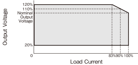
Output Voltage Derating
