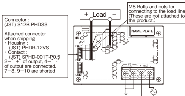
Attached connector when shipping
