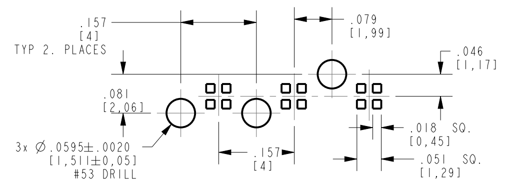
DETAIL A SCALE 8.000
