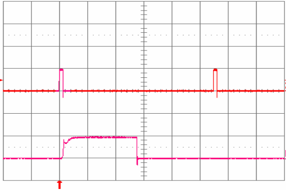
Fig. 28: Load current i_{out1} into a 10 mΩ short circuit on V_{out1} during restart, with V_{out2} open (no load), at V_{in} = 48 V. Ch2 = i_{out1} (20 A/div, 20 ms/div). ChB = i_{out1} (20 A/div, 1 ms/div) is an expansion of the on-time portion of i_{out1} .
