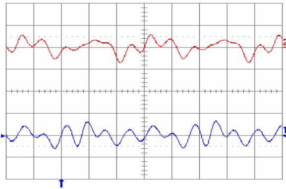
Fig. 30: Output voltage ripple at full rated load current into a resistive load on both outputs with C_o = 1\mu\text{F} (ceramic) and V_{in} = 48 V. Ch2 = V_{out2} , Ch1 = V_{out1} (both 20 mV/div). Time scale: 1 μs/div.
