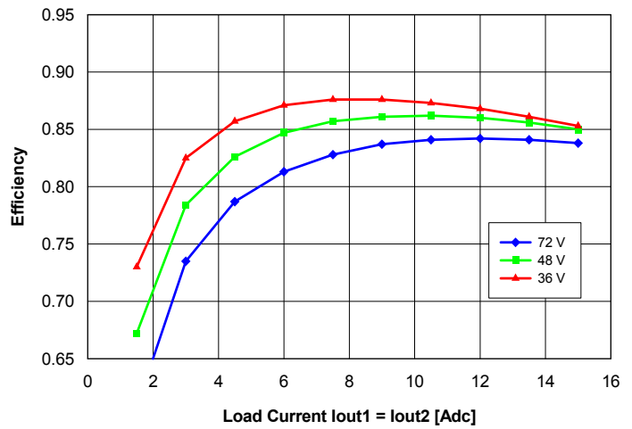
Fig. 17: Efficiency vs. balanced load current (I out1 = I out2 ) and input voltage for converter mounted horizontally with air flowing from pin 3 to pin 1 at a rate of 300 LFM (1.5 m/s) and T a = 25°C.
