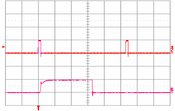
Fig. 29: Load current i_{out2} into a 10 mΩ short circuit on V_{out2} during restart, with V_{out1} open (no load), at V_{in} = 48 V. Ch2 = i_{out2} (20 A/div, 20 ms/div). ChB = i_{out2} (20 A/div, 1 ms/div) is an expansion of the on-time portion of i_{out2} .
