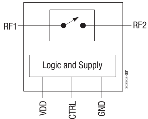
Figure 1. SKY19250-001 Block Diagram
