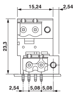
Dimensional drawing
