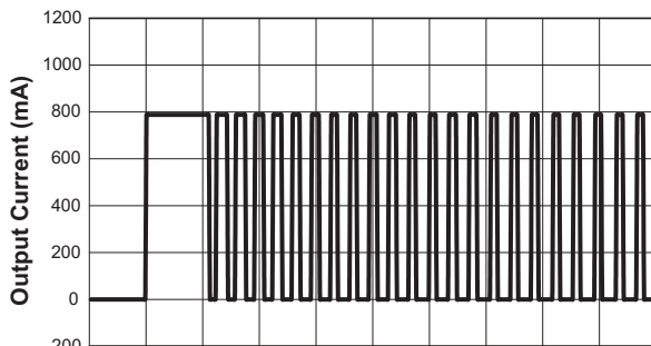
Over-Current Protection
