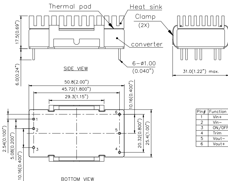
Mechanical Dimensions
