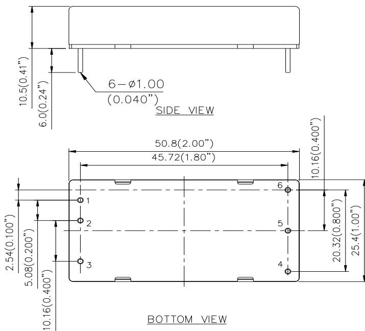
Mechanical Dimensions
