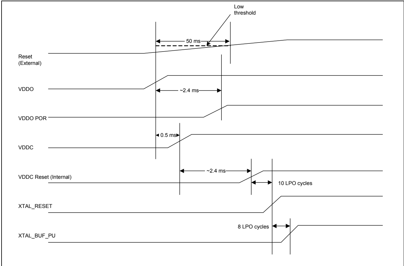
Figure 2: Reset Timing
