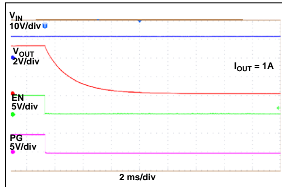
FIGURE 2-29: Enable Turn-Off.
