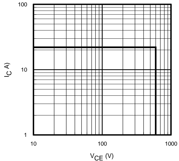
Fig. 4 - Reverse Bias SOA T_J = 175^{\circ}\text{C} ; V_{\text{GE}} = 15\text{V}
