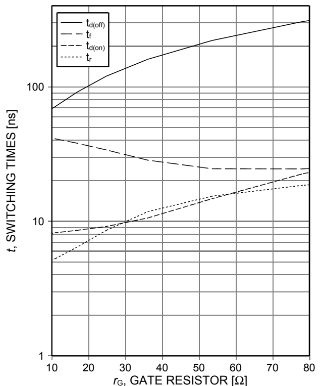
Figure 8. Typical switching times as a function of gate resistor (inductive load, T vj =175°C, V CE =400V, V GE =15/0V, I C =6A, Dynamic test circuit in Figure E)
