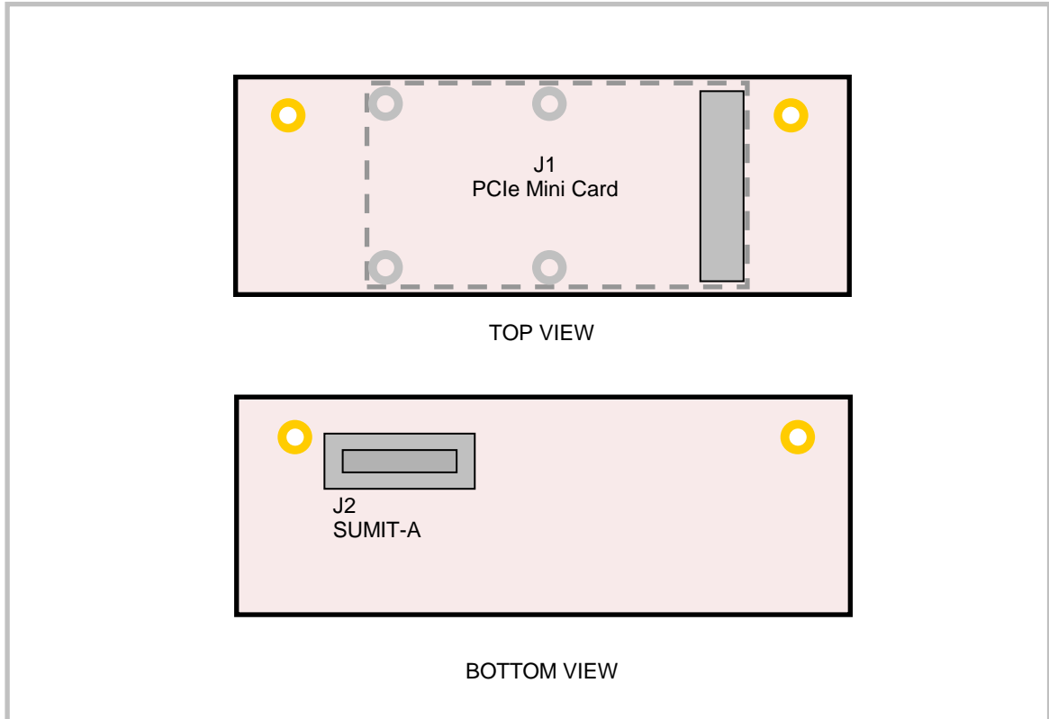
Figure 3. Connector Locations
