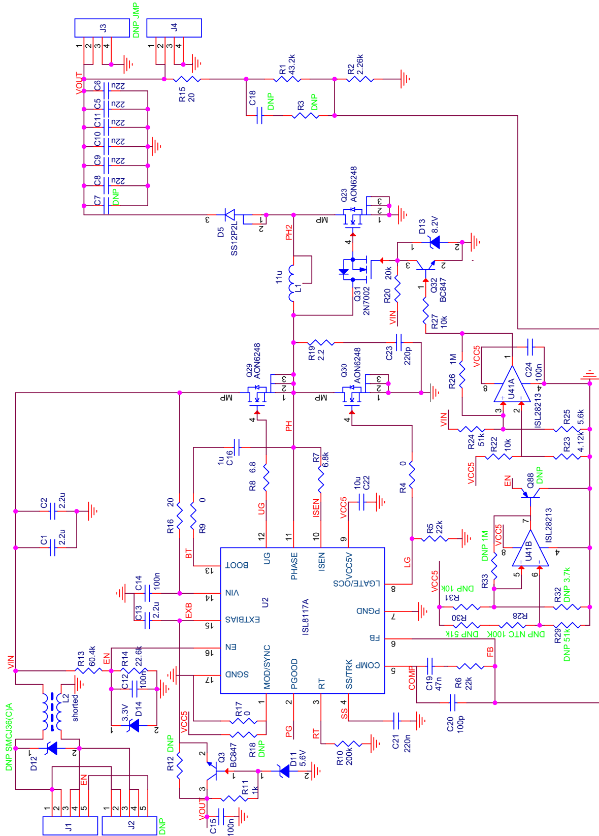
Figure 6. ISL8117ADEMO4Z Schematic
