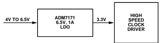
Figure 67. Clock Driver Power
