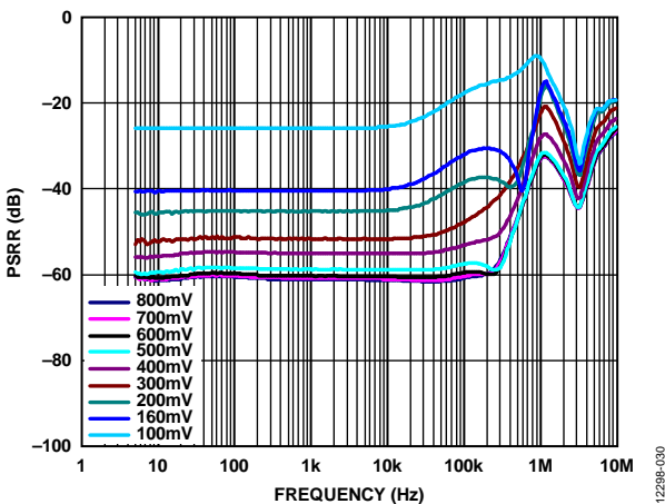
Figure 30. Power Supply Rejection Ratio (PSRR) vs. Frequency, V_{OUT} = 3 V , 1 A Load Current, Various Headroom Voltages
