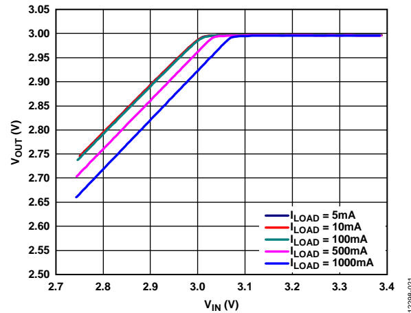
Figure 21. Output Voltage ( V_{OUT} ) vs. Input Voltage ( V_{IN} ) in Dropout, V_{OUT} = 3V
