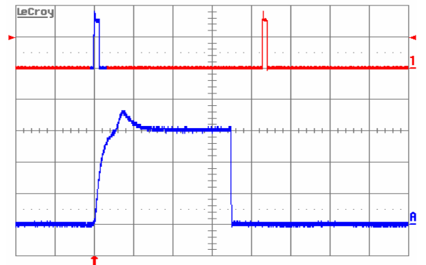
Figure 15. Load current (top trace, 20 A/div., 50 ms/div.) into a 10 \text{ m}\Omega short circuit during restart, at V_{in} = 48 \text{ V} . Bottom trace (10 A/div., 2 ms/div.) is an expansion of the on-time portion of the top trace
