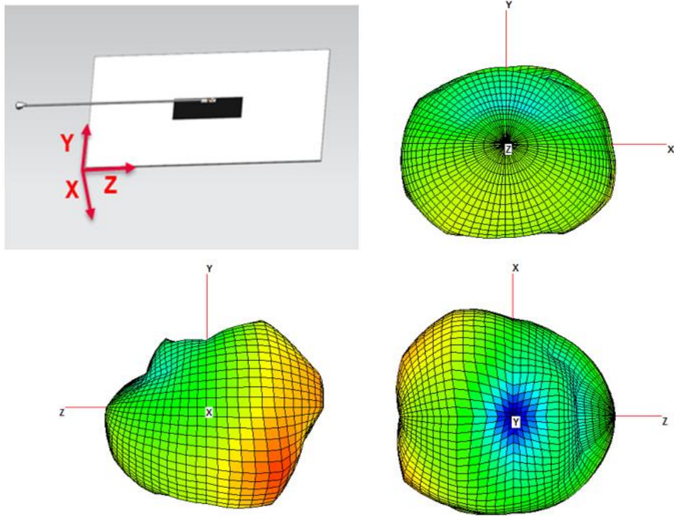
FIGURE 4.5.3 3D RADIATION PATTERN OF ANTENNA AT 2.45GHZ IN FREE SPACE
