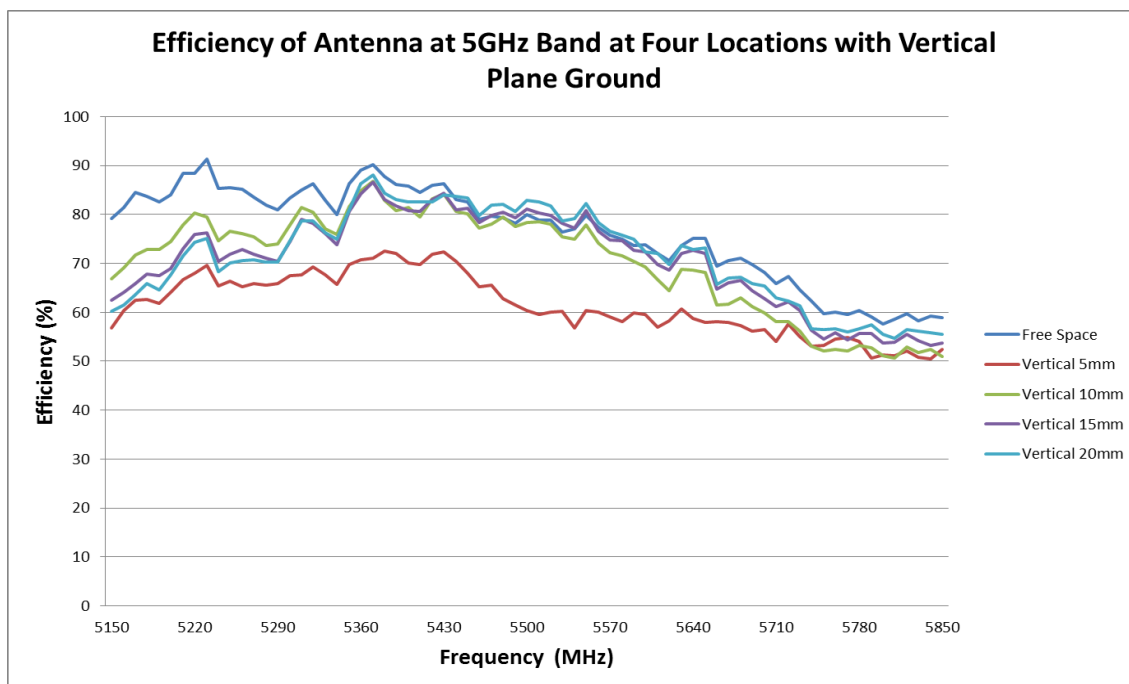
FIGURE 6.2.5 EFFICIENCY OF ANTENNA AT WIFI 5GHZ BAND AT FOUR LOCATIONS WITH VERTICAL PLANE GROUND
