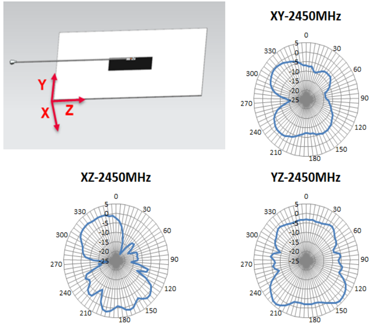
FIGURE 4.5.1 2D RADIATION PATTERN OF ANTENNA AT 2.45GHZ IN FREE SPACE
