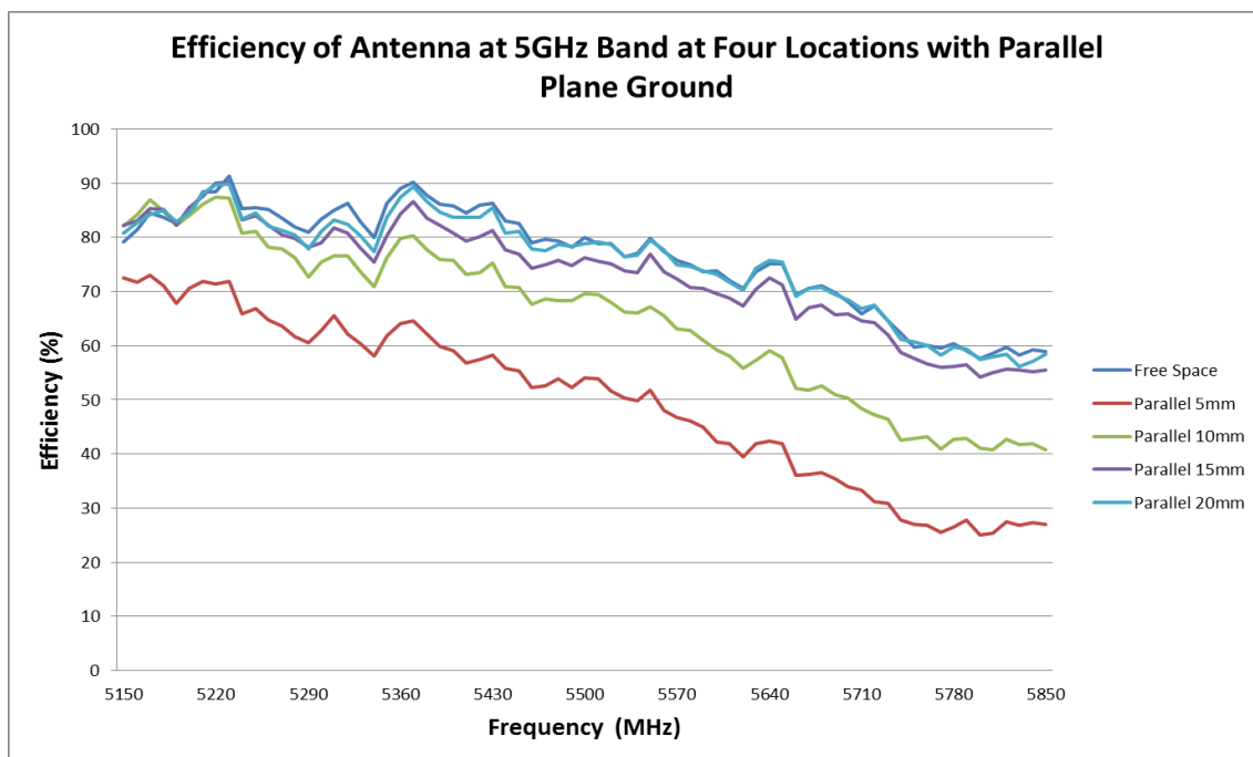
FIGURE 6.1.5 EFFICIENCY OF ANTENNA AT WIFI 5GHZ BAND AT FOUR LOCATIONS WITH PARALLEL PLANE GROUND
