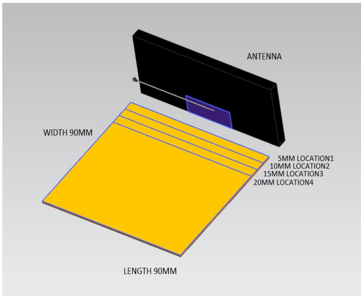
FIGURE 6.2.1 FOUR LOCATIONS WITH VERTICAL PLANE GROUND
