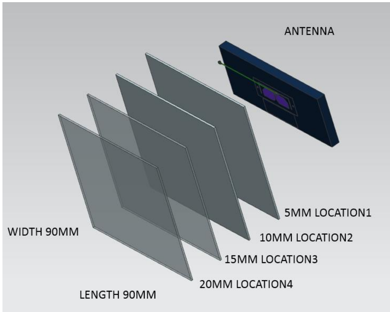
FIGURE 6.1.1 FOUR LOCATIONS WITH PARALLEL PLANE GROUND
