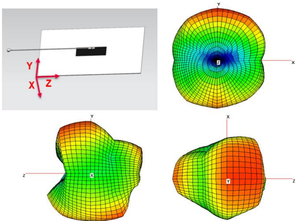
FIGURE 4.5.4 3D RADIATION PATTERN OF ANTENNA AT 5.45GHZ IN FREE SPACE
