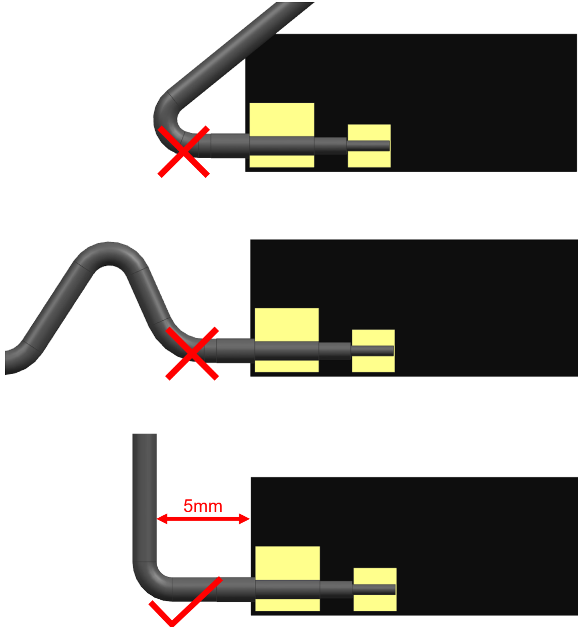
FIGURE 5.2 CABLE BENDING
