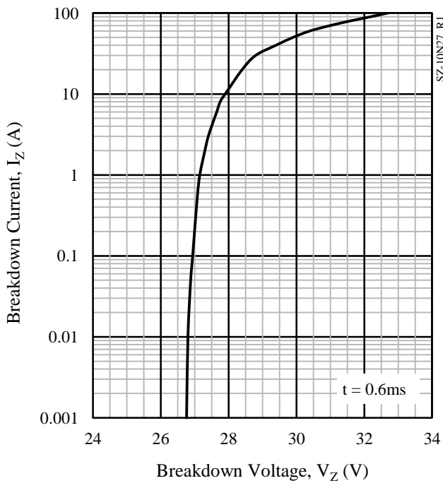
Figure 3-7 I_Z - V_Z typical characteristics
