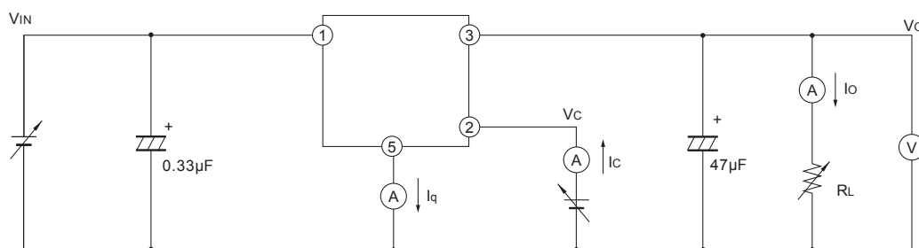
Fig.1 Test Circuit
