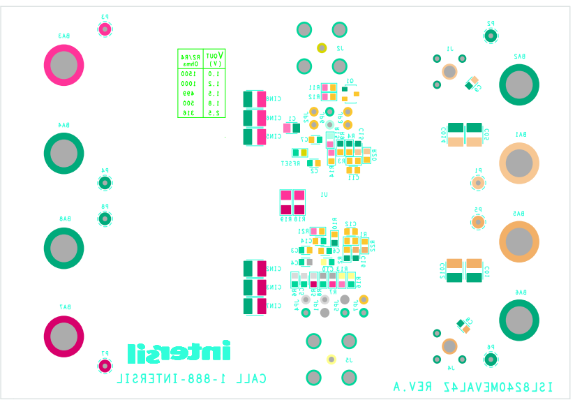
FIGURE 8. BOTTOM SILKSCREEN
