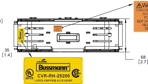
HM25200-1CR WITH CVR-RH-25200 INSTALLED
