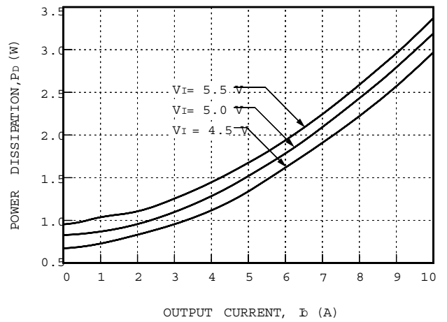
Figure 46. NH033G-L Typical Power Dissipation vs. Output Current, TA = 25 °C
