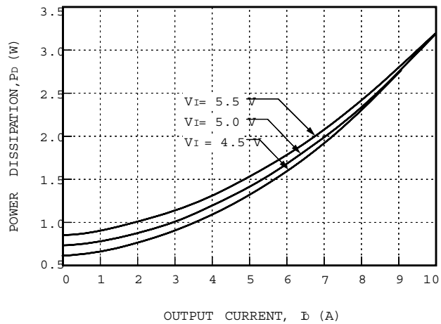
Figure 44. NH033S1R8-L Typical Power Dissipation vs. Output Current, TA = 25 °C
