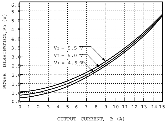
Figure 43. NH050M-L Typical Power Dissipation vs. Output Current, TA = 25 °C
