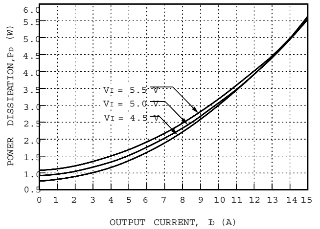
Figure 45. NH050S1R8-L Typical Power Dissipation vs. Output Current, TA = 25 °C
