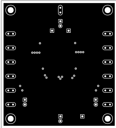
PCB Layout—Solder Side
