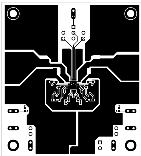
PCB Layout—Component Side
