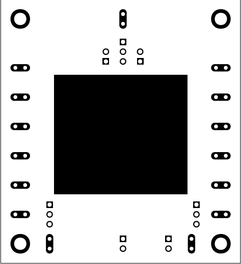
Component Placement Guide—Bottom Solder Mask
