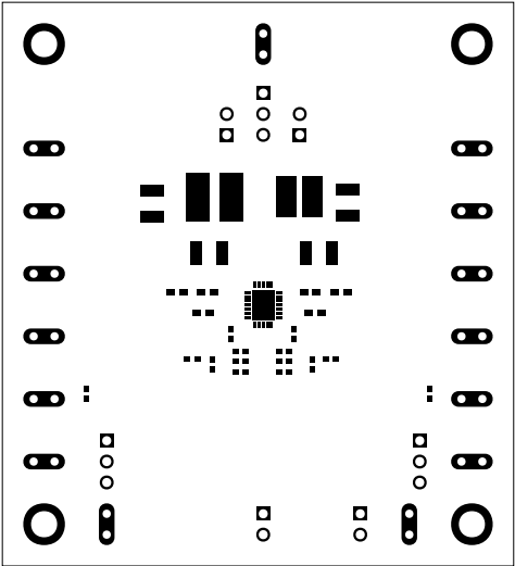
PCB Layout—Solder Mask
