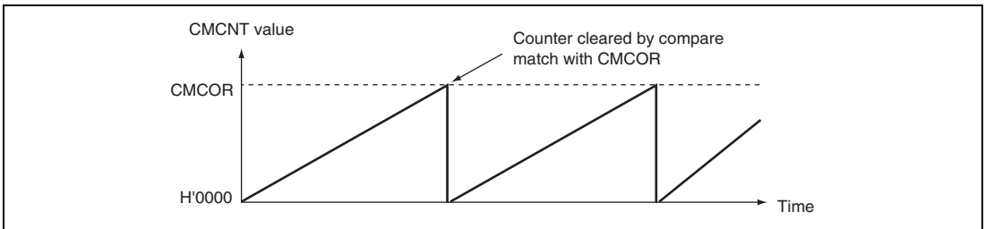
Figure 12.2 Counter Operation
