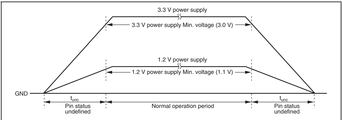
Figure 31.1 Power-on/Power-off Sequence
