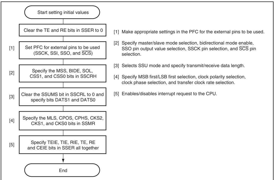
Figure 16.4 Example of Initial Settings in SSU Mode
