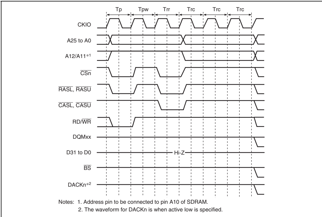
Figure 9.28 Auto-Refresh Timing
