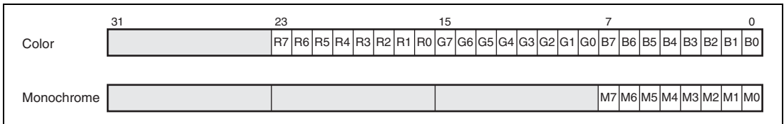
Figure 24.3 Color-Palette Data Format
