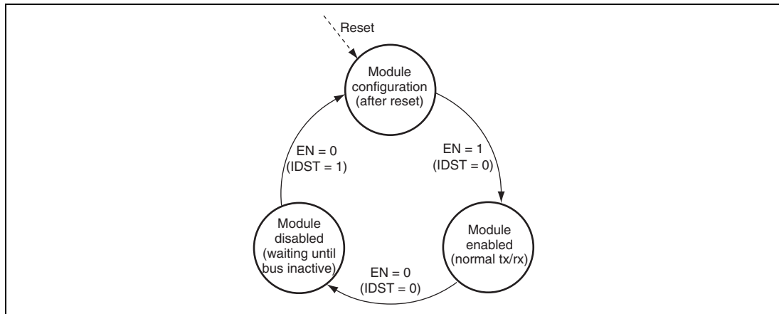
Figure 18.19 Operation Modes
