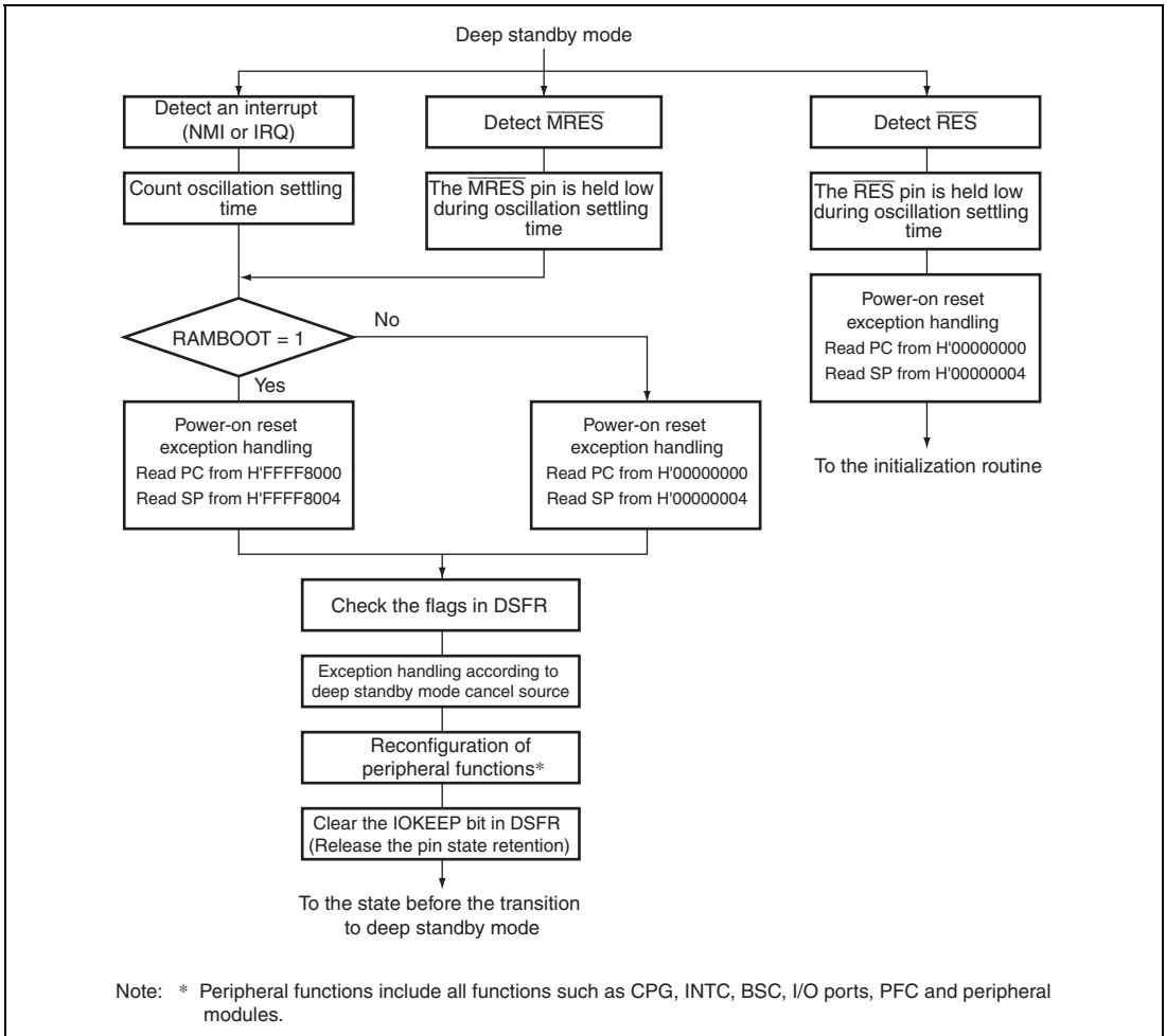
Figure 28.3 Flowchart of Canceling Deep Standby Mode
