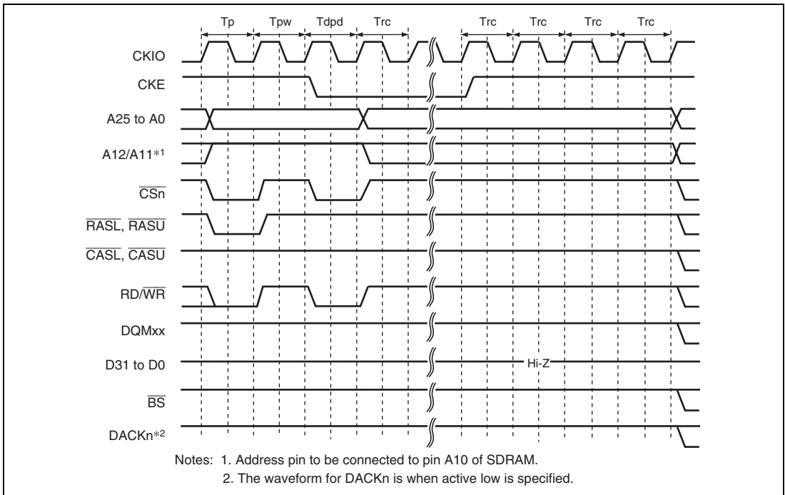
Figure 9.34 Deep Power-Down Mode Transition Timing
