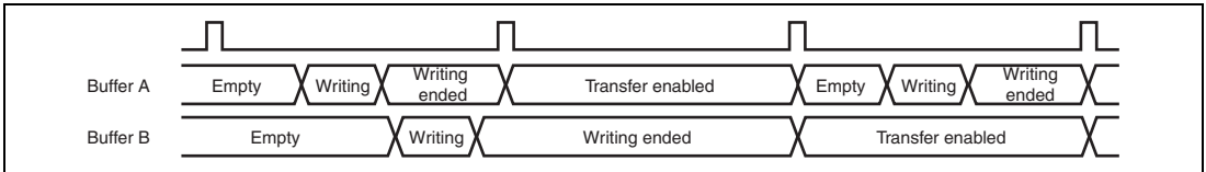
Figure 23.18 Example of Buffer Flush Function Operation
