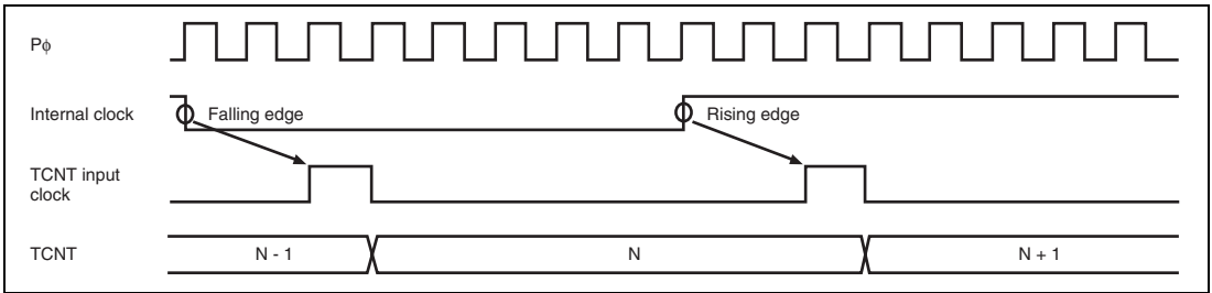
Figure 11.78 Count Timing in Internal Clock Operation
