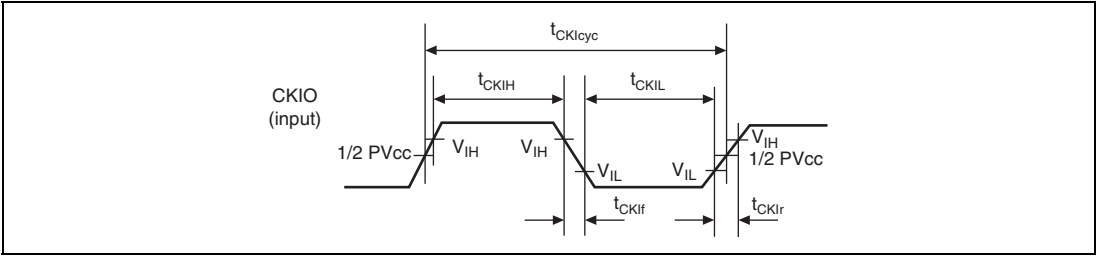
Figure 31.3 CKIO Clock Input Timing
