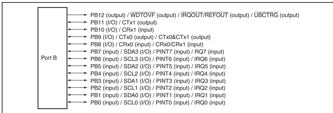
Figure 26.2 Port B
