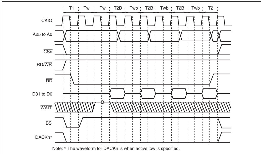
Figure 9.35 Burst ROM Access Timing (Clocked Asynchronous)
