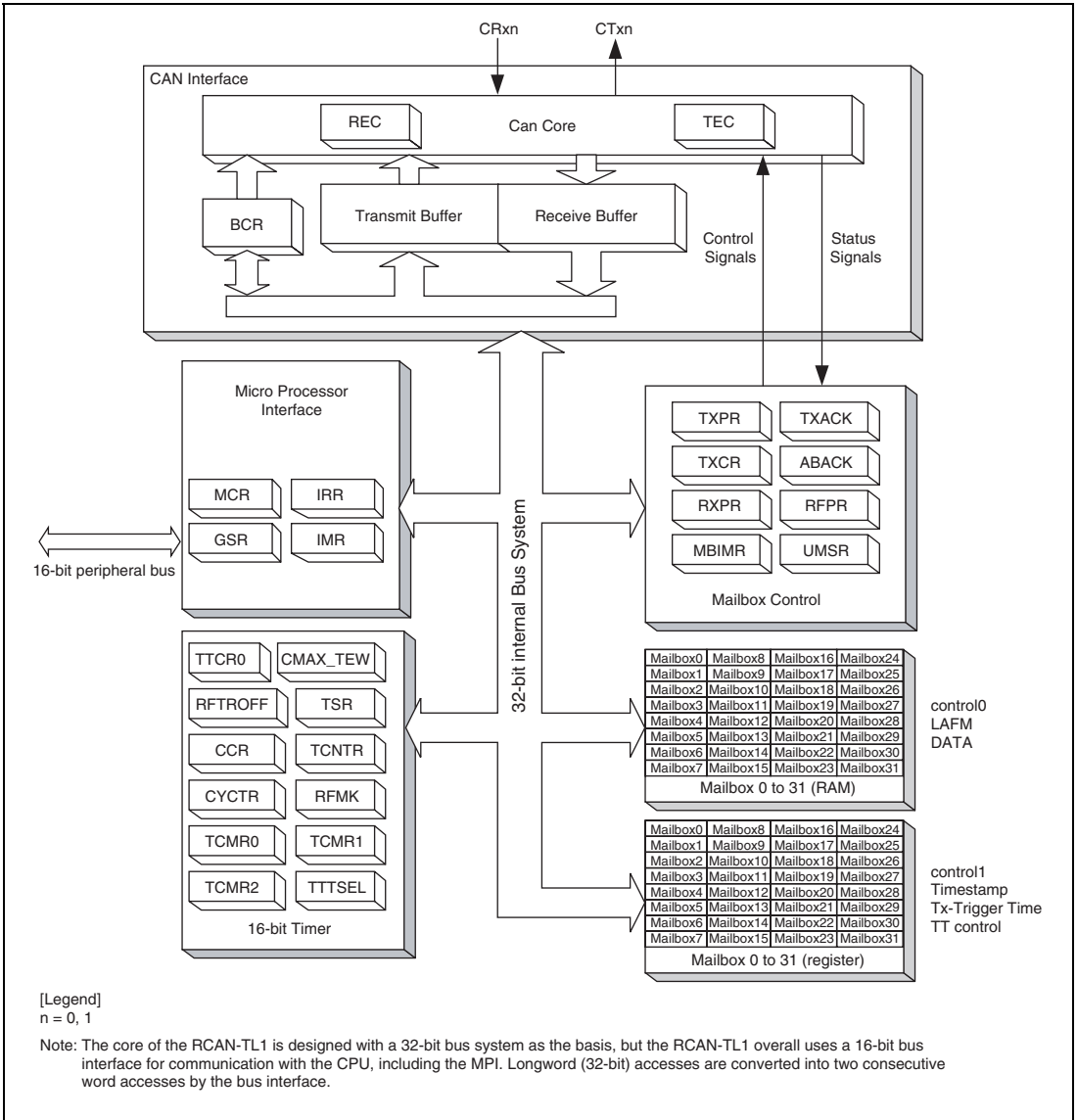
Figure 19.1 RCAN-TL1 architecture
