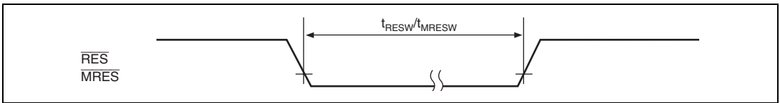
Figure 31.9 Reset Input Timing
