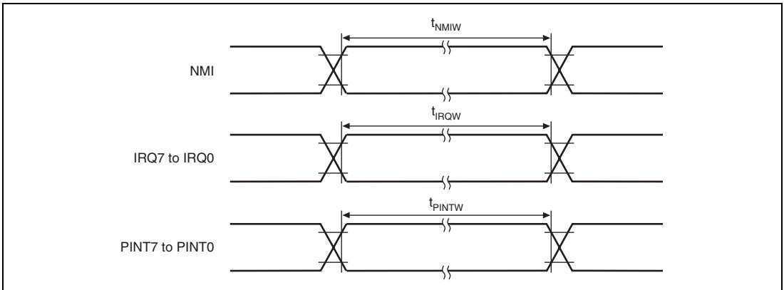
Figure 31.10 Interrupt Signal Input Timing
