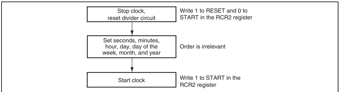
Figure 14.2 Setting Time
