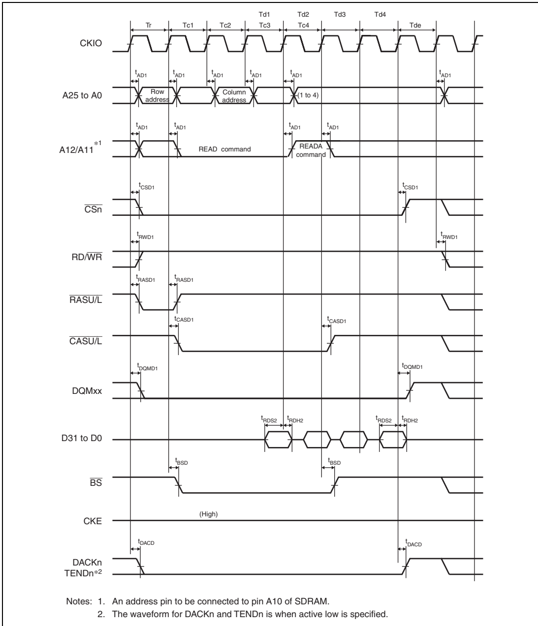
Figure 31.24 Synchronous DRAM Burst Read Bus Cycle (Four Read Cycles) (Auto Precharge, CAS Latency 2, WTRCD = 0 Cycle, WTRP = 1 Cycle)
