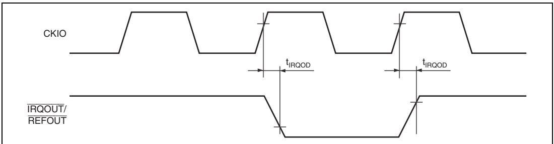
Figure 31.11 Interrupt Signal Output Timing
