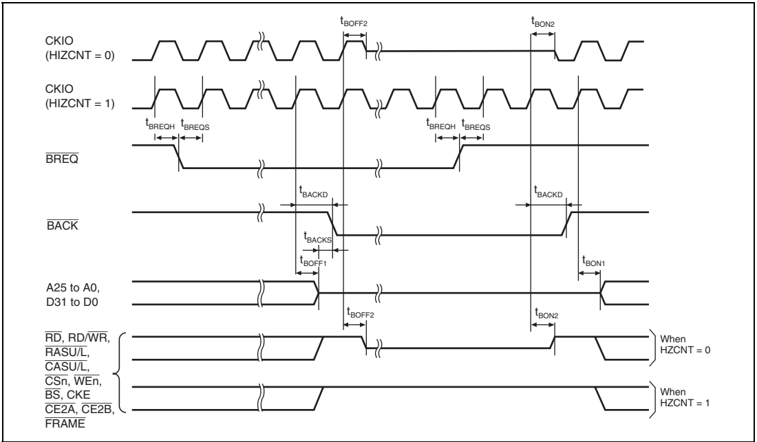
Figure 31.12 Bus Release Timing
