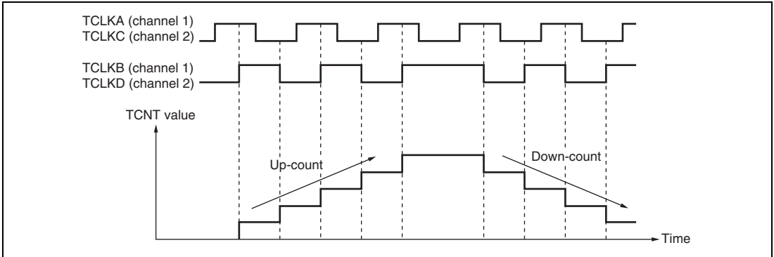
Figure 11.33 Example of Phase Counting Mode 4 Operation
