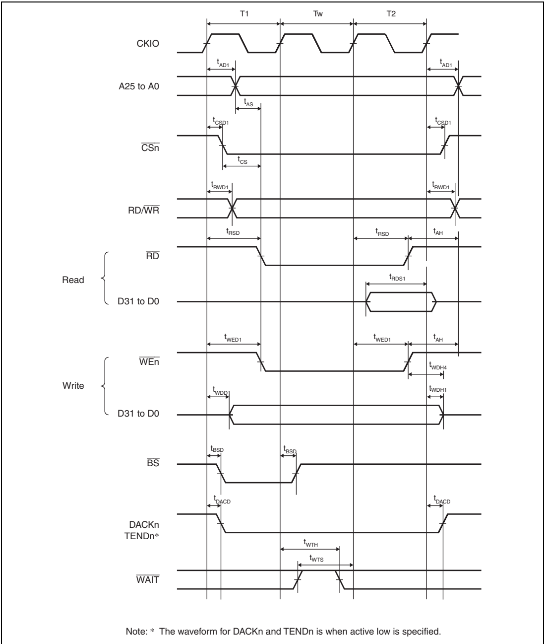
Figure 31.14 Basic Bus Timing for Normal Space (One Software Wait Cycle)
