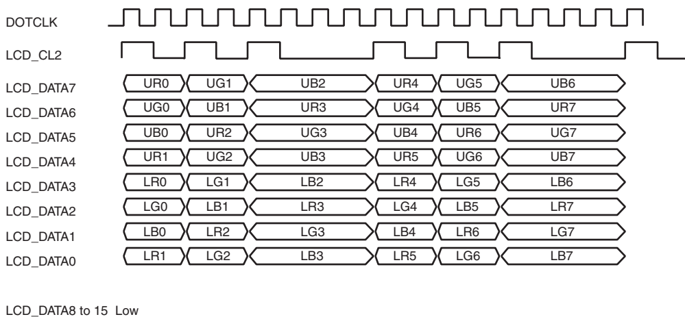
Figure 24.18 Clock and LCD Data Signal Example (DSTN Color 8-Bit Data Bus Module)
