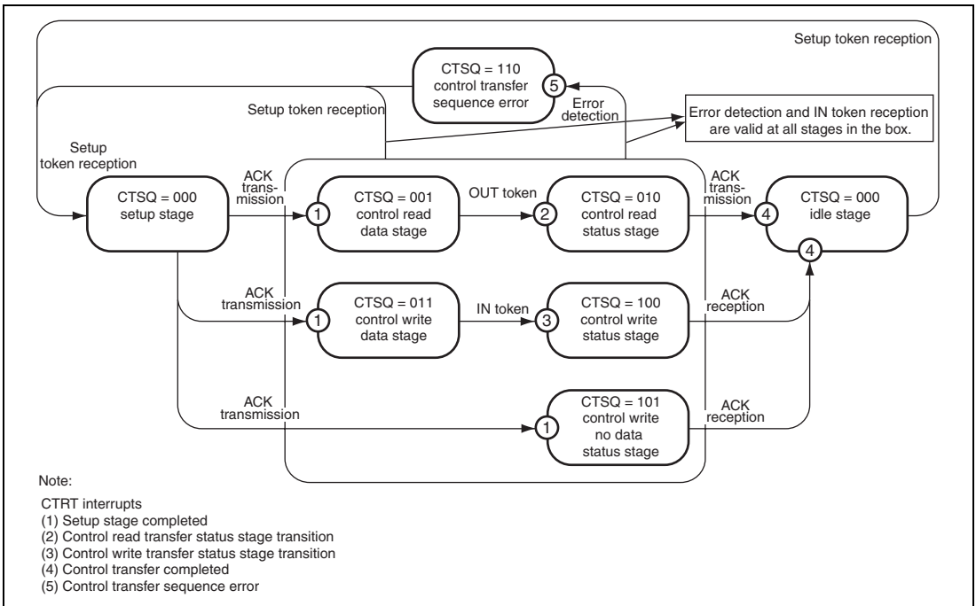
Figure 23.7 Control Transfer Stage Transitions
