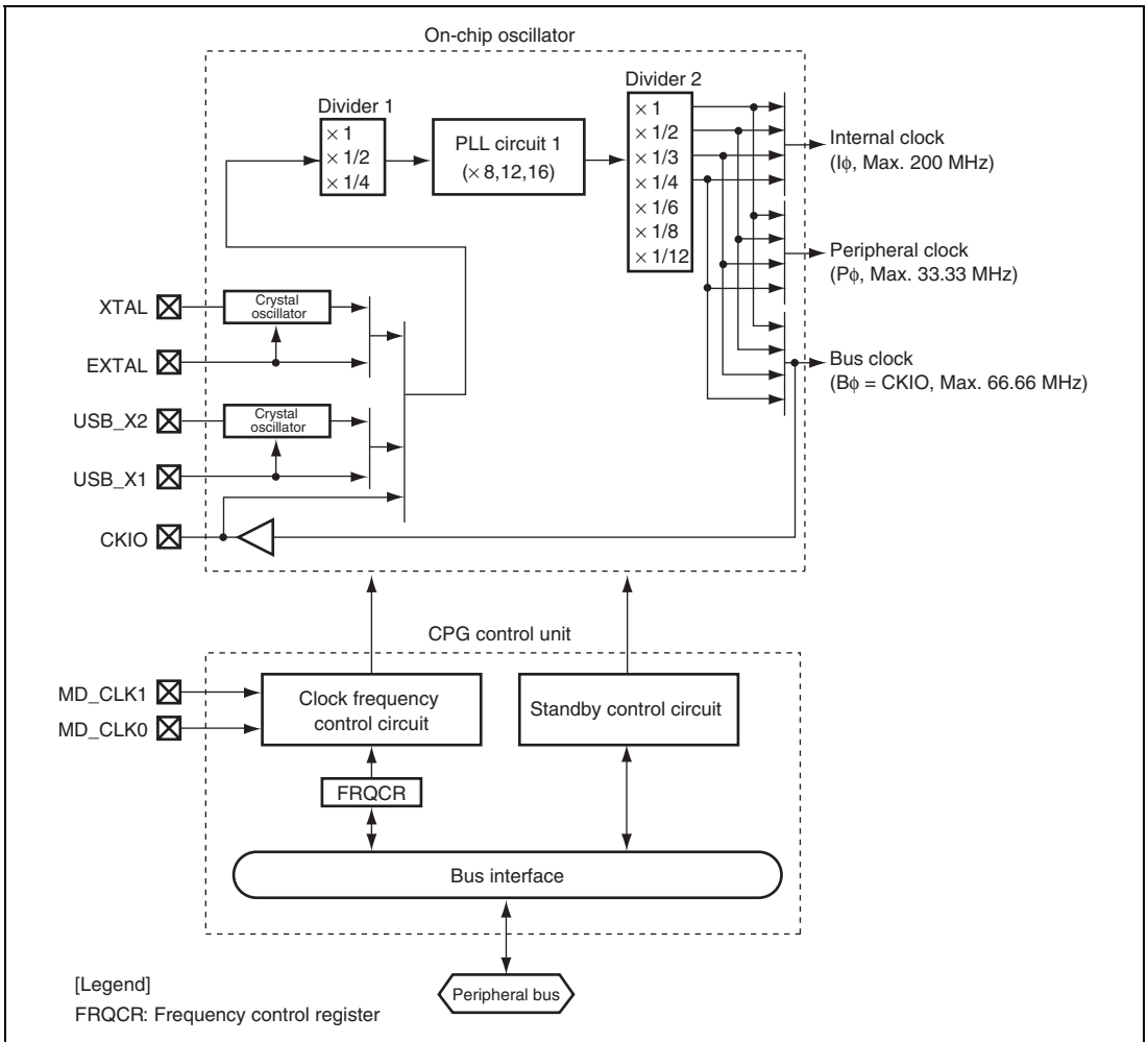
Figure 4.1 Block Diagram of Clock Pulse Generator
