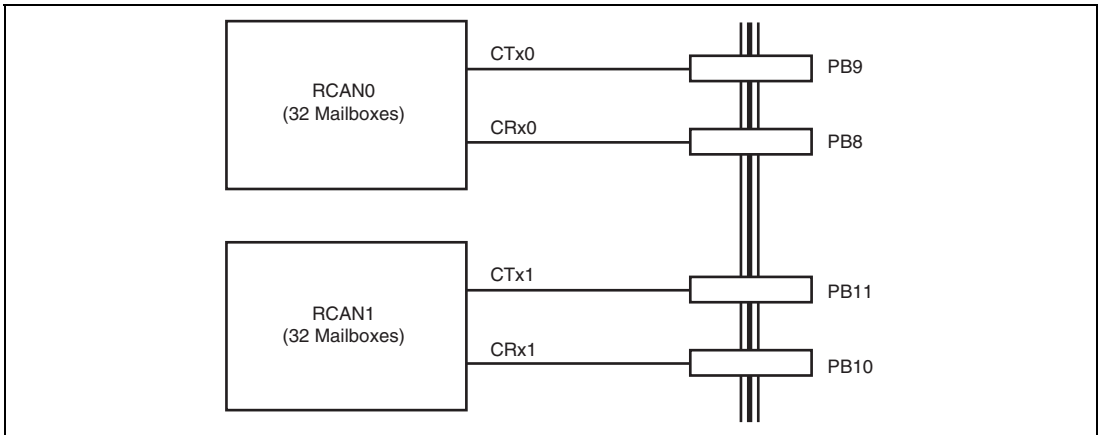
Figure 19.28 Connection Example when Using RCAN-TL1 as 2-Channel Module (32 Mailboxes × 2 Channels)
