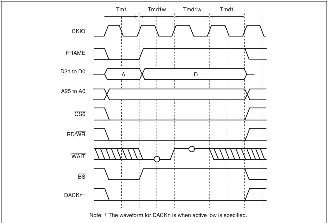
Figure 9.49 Burst MPX Space Access Timing (Single Write, Software Wait 1, Hardware Wait 1)
