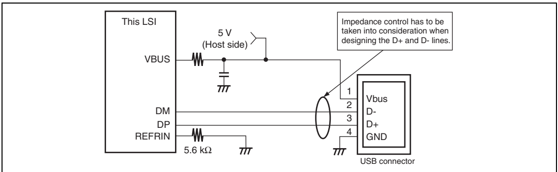
Figure 23.1 UBS Connector Connection
