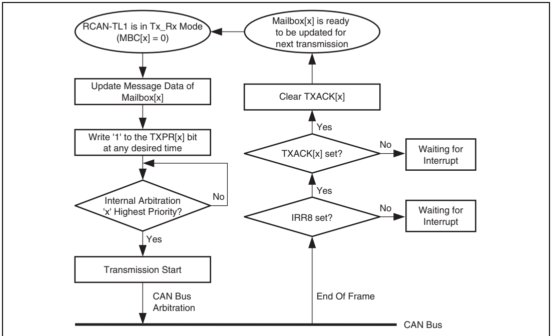
Figure 19.16 Transmission request
