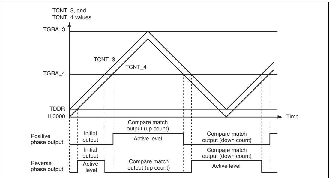
Figure 11.2 Complementary PWM Mode Output Level Example
