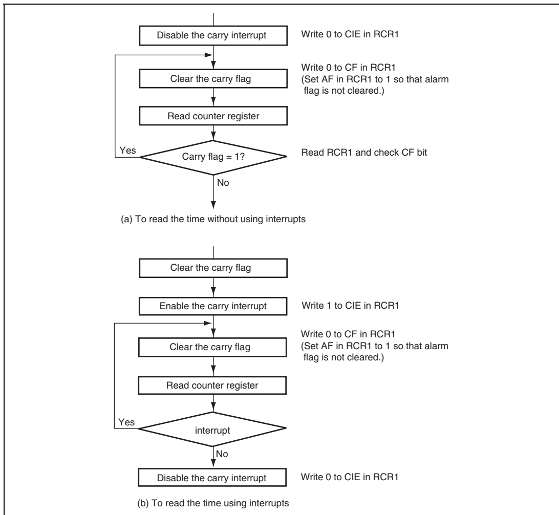
Figure 14.3 Reading Time
