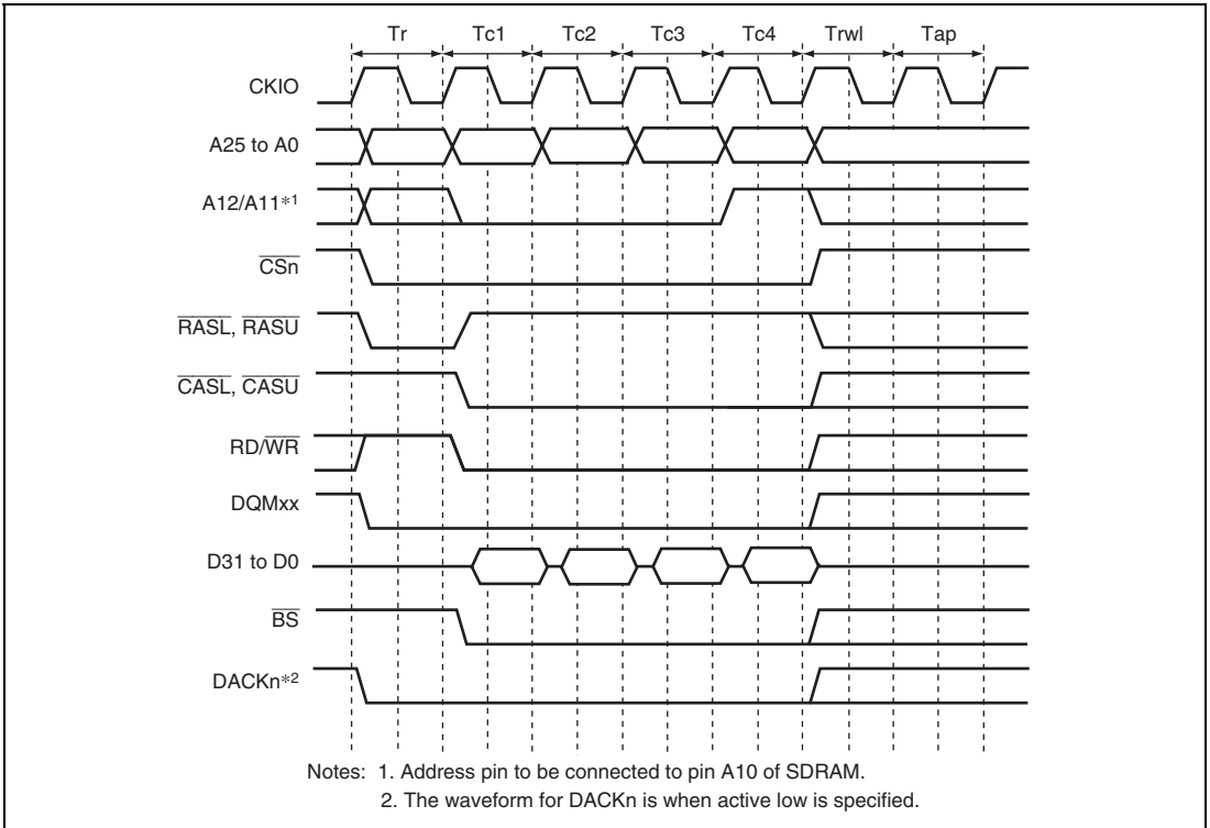
Figure 9.20 Basic Timing for Burst Write (Auto Pre-Charge)
