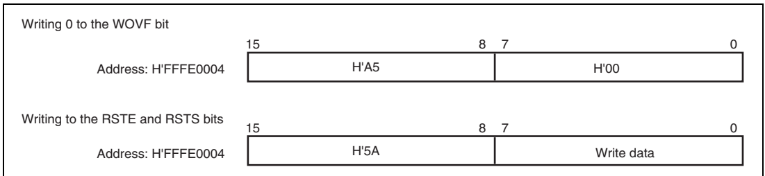
Figure 13.3 Writing to WRCSR
