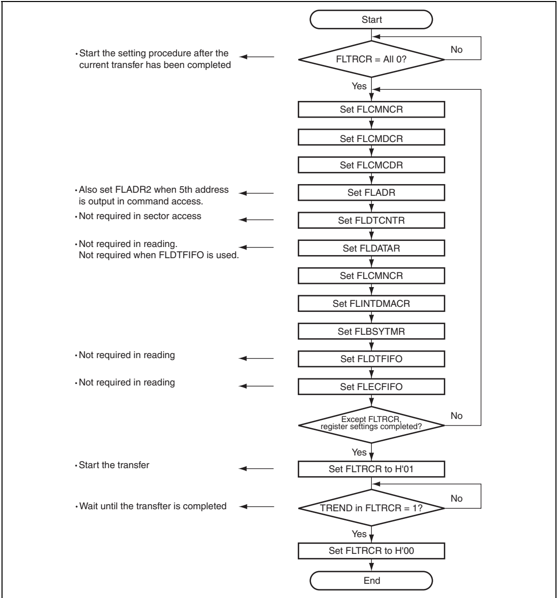
Figure 22.3 Register Setting Flow
