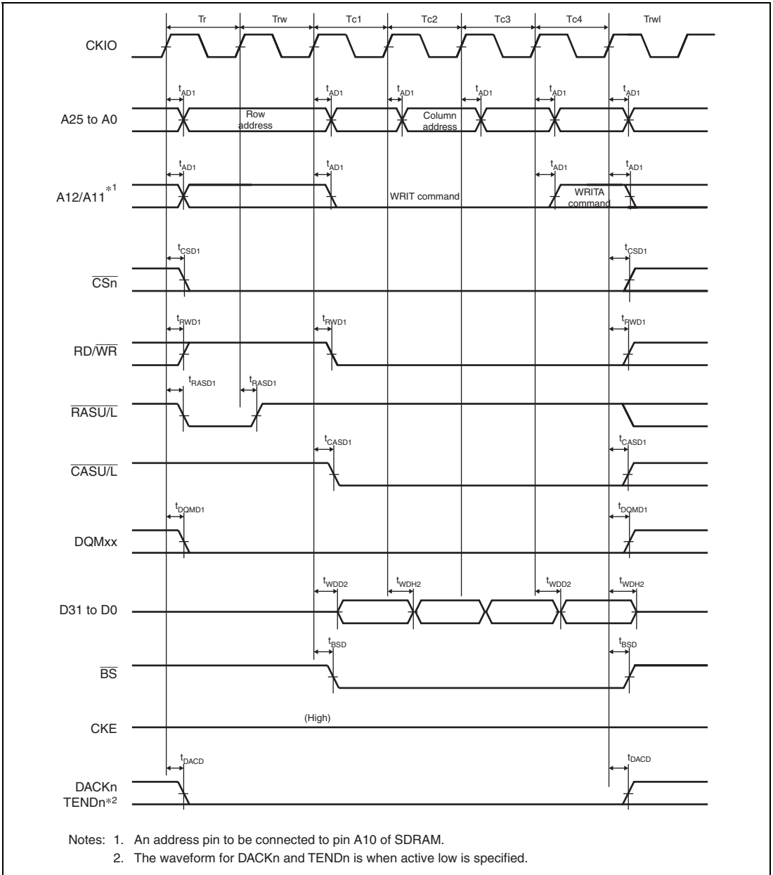
Figure 31.29 Synchronous DRAM Burst Write Bus Cycle (Four Write Cycles) (Auto Precharge, WTRCD = 1 Cycle, TRWL = 1 Cycle)
