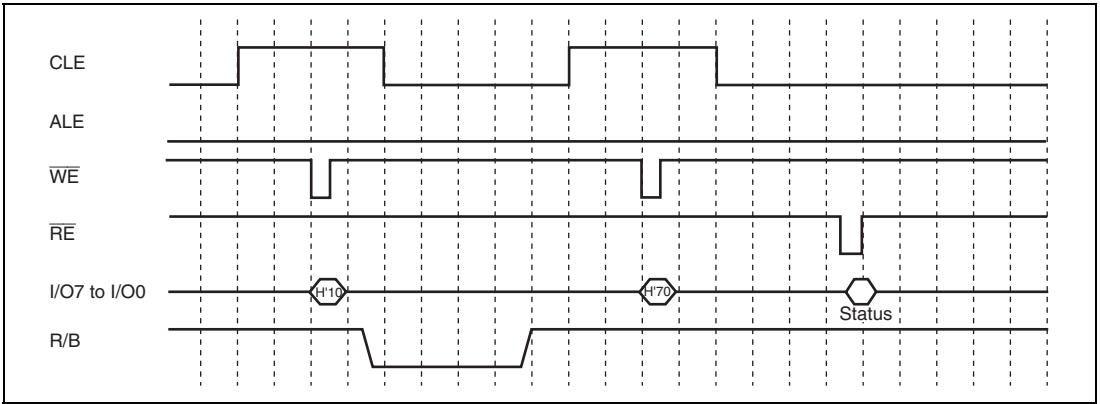
Figure 22.10 Programming Operation Timing for NAND-Type Flash Memory (2)
