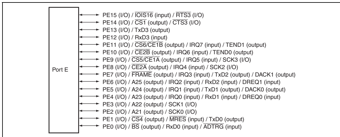
Figure 26.5 Port E
