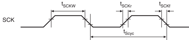
Figure 31.51 SCK Input Clock Timing
