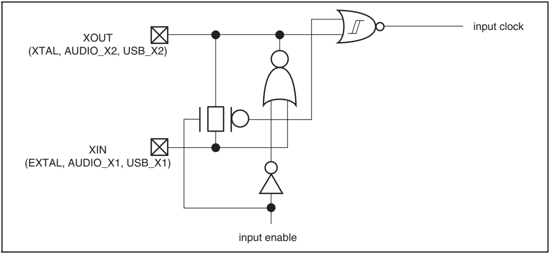
Figure 1.3 (13) Simplified Circuit Diagram (Oscillation Buffer 1)
