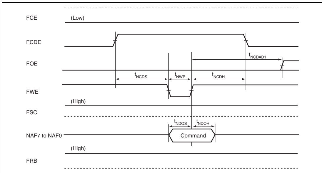
Figure 31.69 NAND Type Flash Memory Command Issuance Timing
