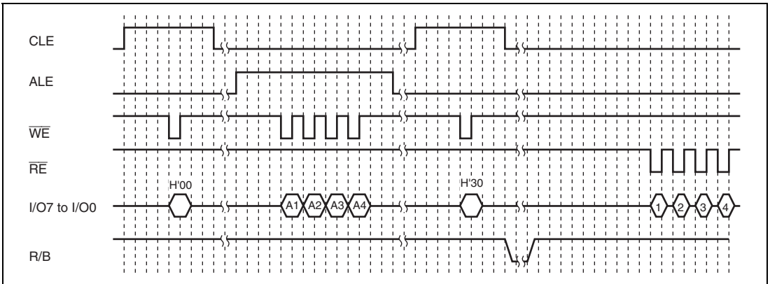
Figure 22.11 Read Operation Timing for NAND-Type Flash Memory
