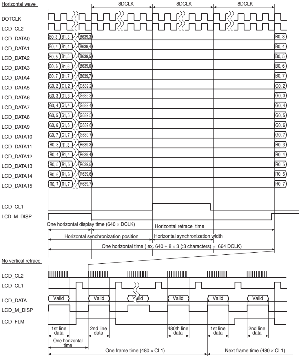
Figure 24.23 Clock and LCD Data Signal Example (16-Bit Interface Color 640 × 480)
