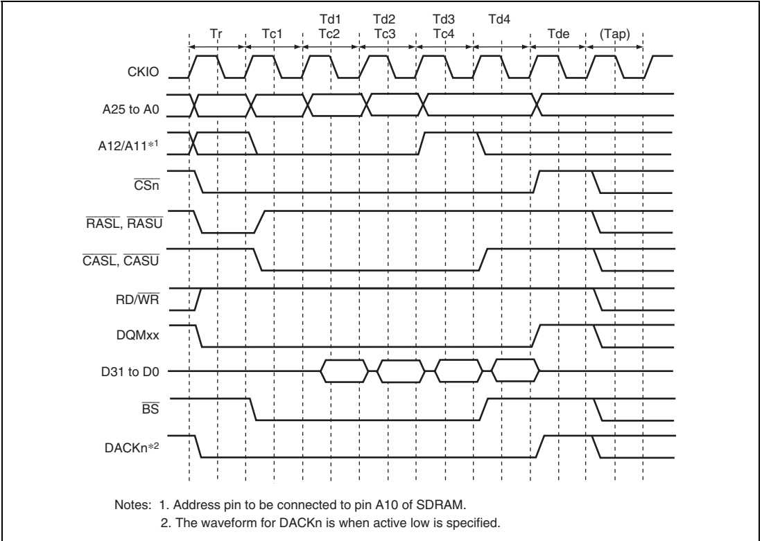
Figure 9.17 Burst Read Basic Timing (CAS Latency 1, Auto Pre-Charge)
