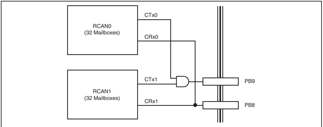
Figure 19.29 Connection Example when Using RCAN-TL1 as 1-Channel Module (64 Mailboxes × 1 Channel)
