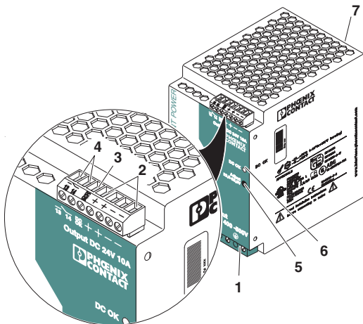
Figure 1 Operating elements
