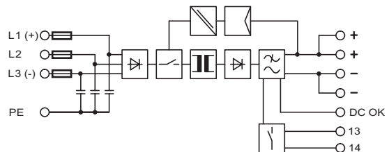
Figure 2 Block diagram
