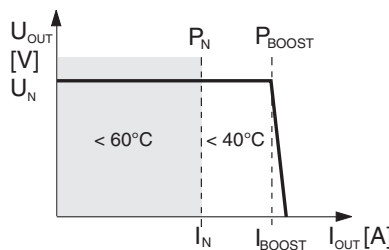
Figure 13 Output characteristic curve
